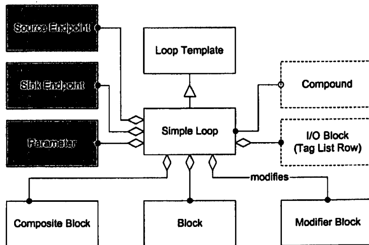
Figure 89 - Simple Loop object model
